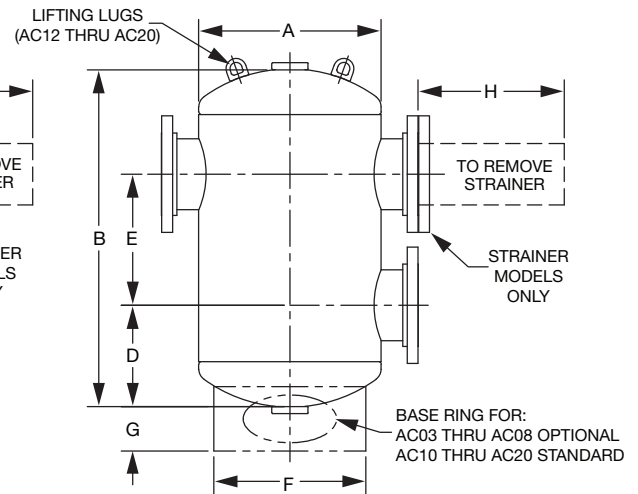
AC03F – AC20F (FLANGED CONNECTIONS – ANSI CL.150 RF SO)
